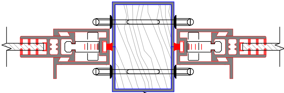
VERTICAL MULLION (VINYL SLEEVES OVER WOOD POST SECURED TO HEAD & SILL w/ POCKET SCREWS)
