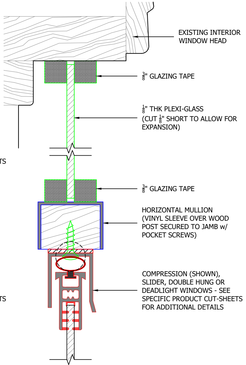
HORIZONTAL MULLION (VINYL SLEEVE OVER WOOD POST SECURED TO JAMB w/ POCKET SCREWS)
