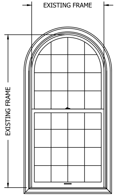
EXISTING WINDOW (OVERSIZED - SINGLE HUNG w/ ARCH TOP)
