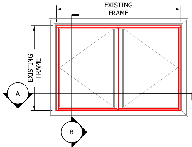
SLIDING STORM WINDOW OVER DOUBLE CASEMENT
