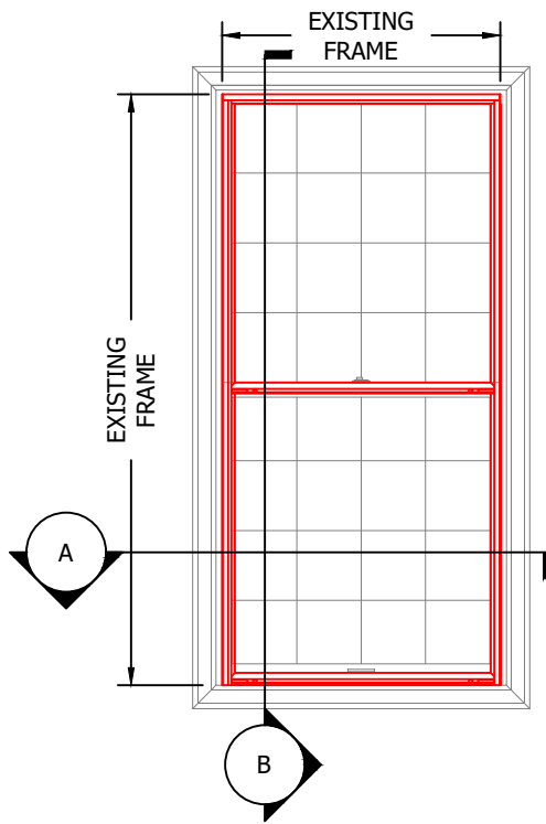
DOUBLE HUNG STORM WINDOW
